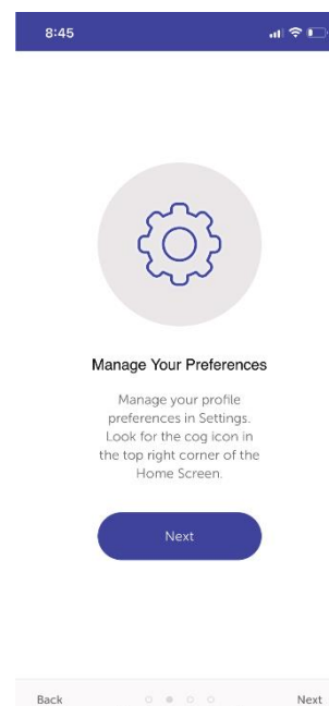
Figure 9 Select 'Next'
