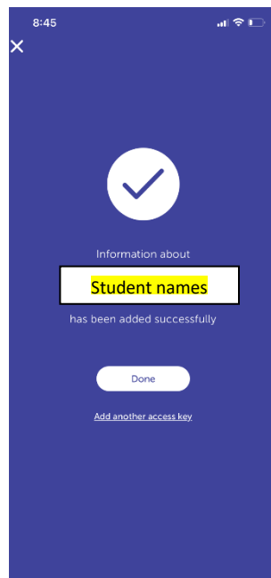
Figure 8 Link successful!
